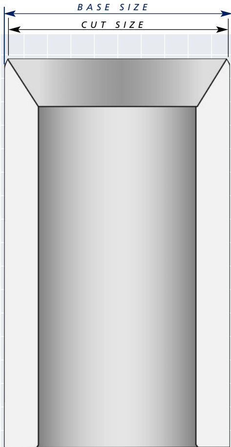
PUNCH CROSS SECTION
